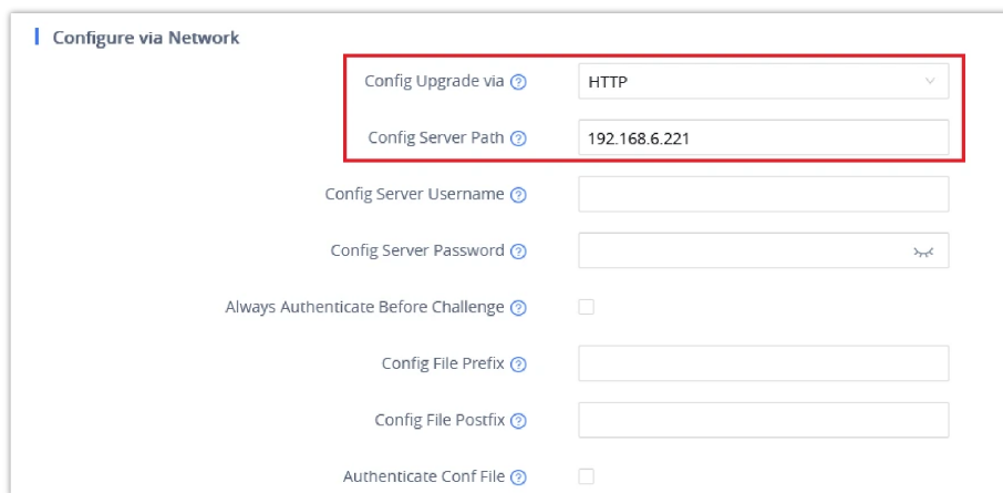
GRP261x Upgrade and Provisioning Settings
