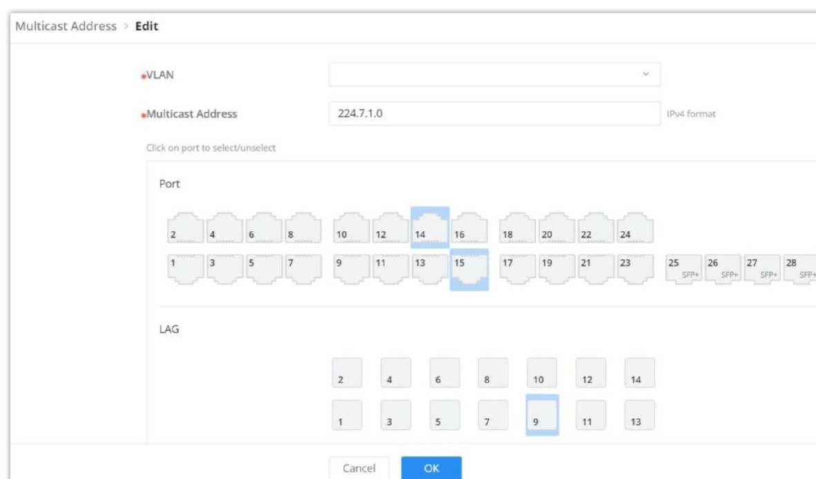
Add IGMP Snooping Multicast Address
