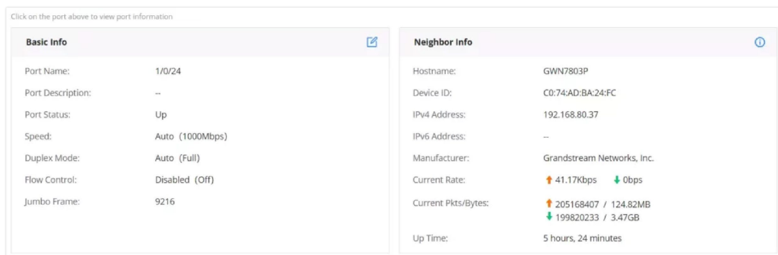
Port Info page 2
