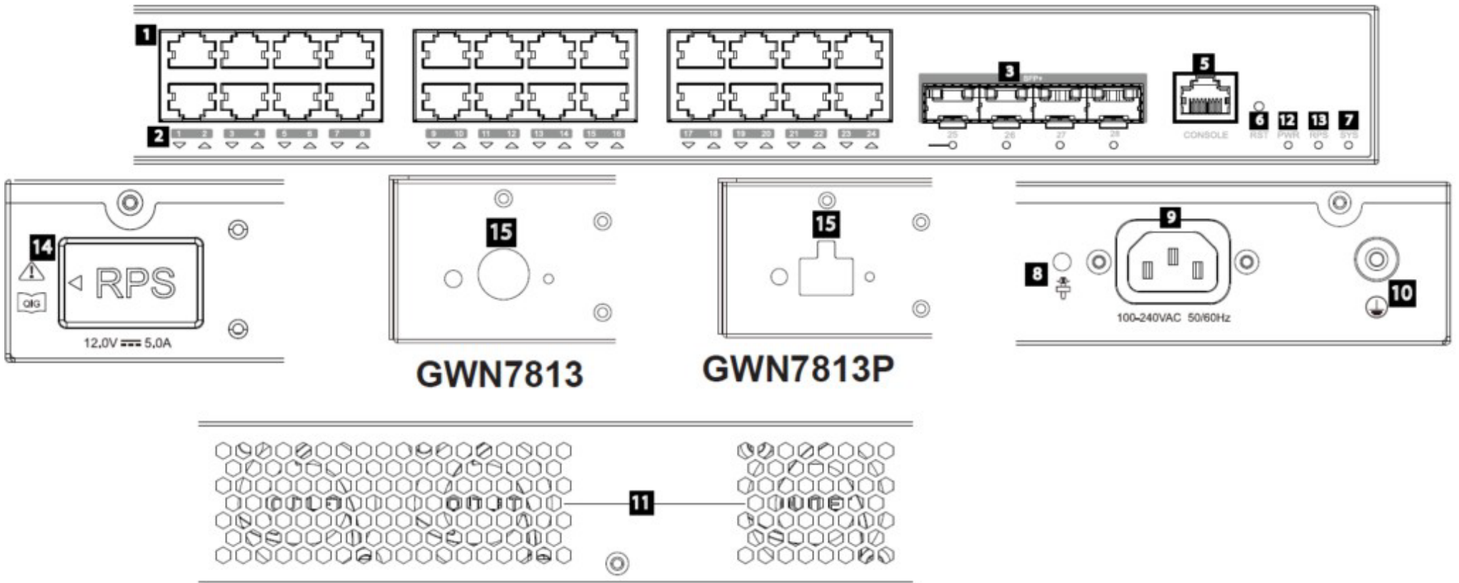
GWN7813GWN7813P Ports
