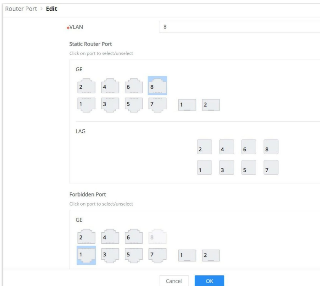
IGMP Snooping Router Port add or edit
