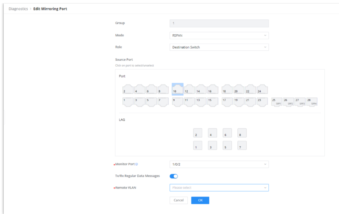
Destination Switch Role RSPAN
