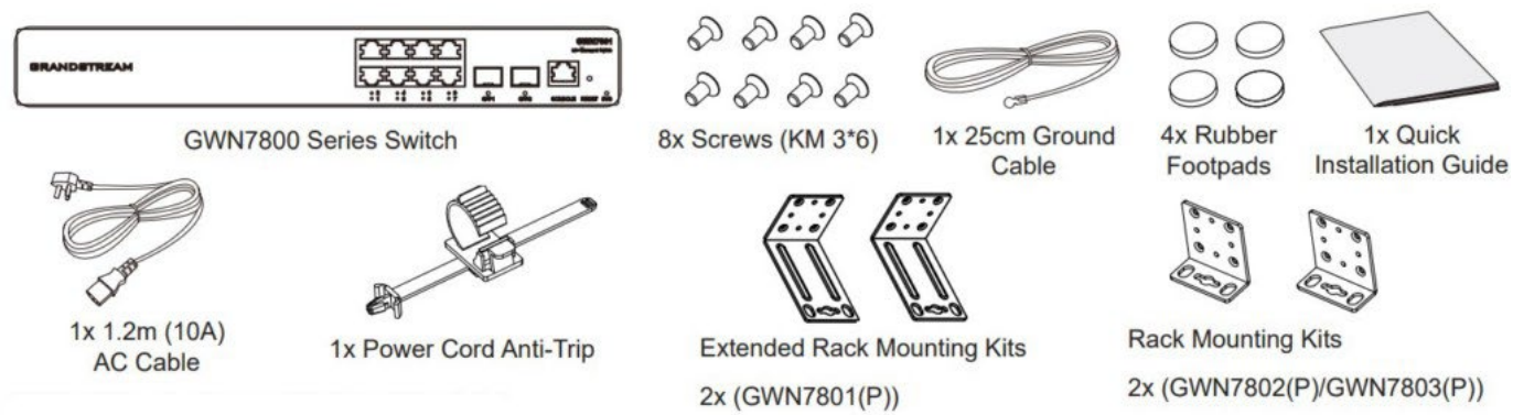
GWN780x Package Contents
