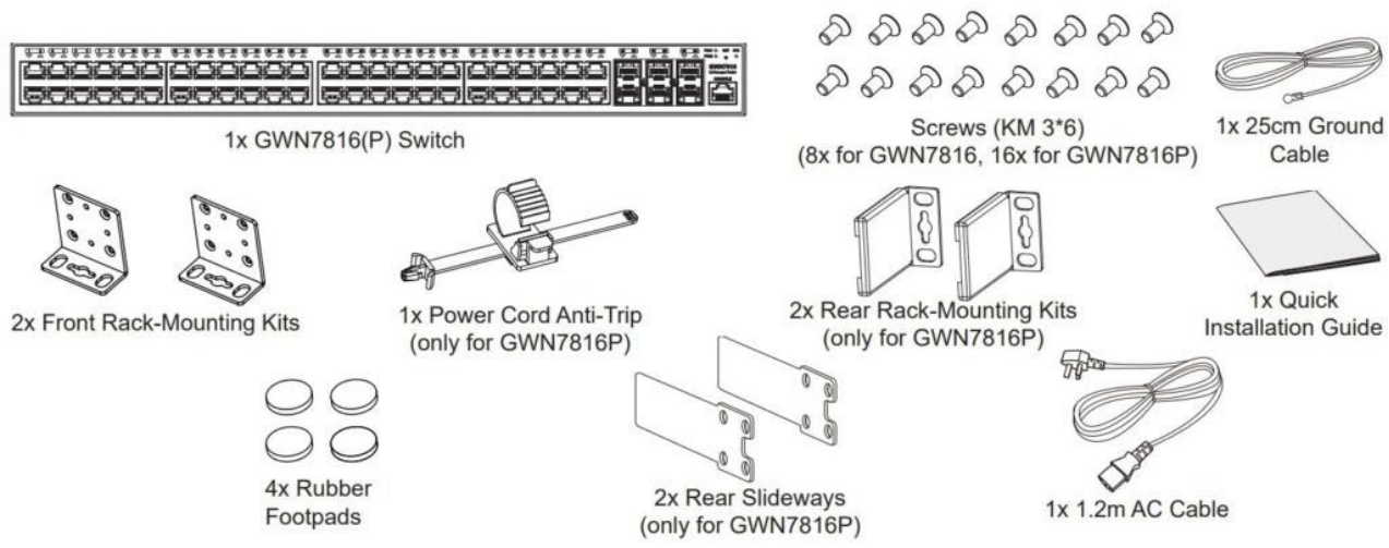
GWN7816P Package Content
