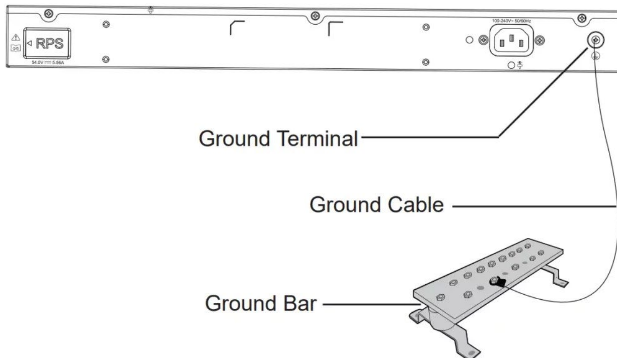
Grounding the Switch
