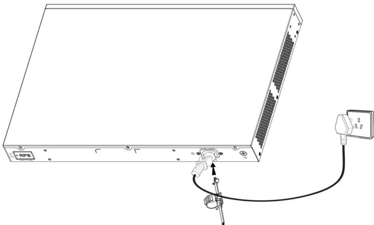
Connecting Power Cord Anti trip
