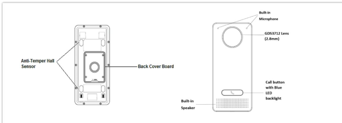
GDS3712 Front and Back View
