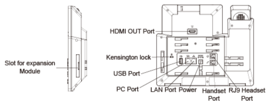
Figure 4: GXV3350 Back / Side View
