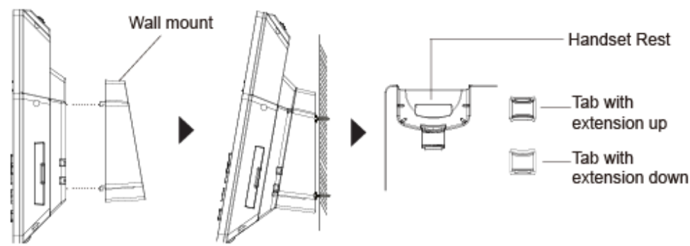
Figure 3: Tab on The Handset Cradle
