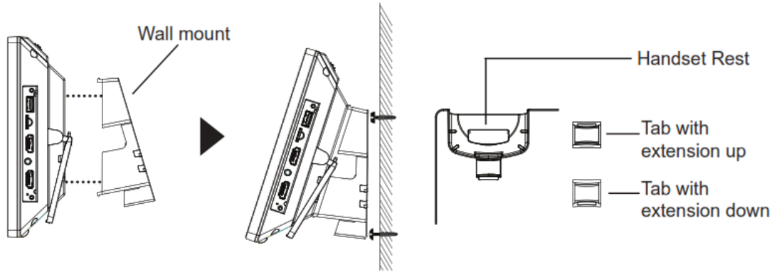
GXV3380 Phone Setup – Wall Mount
